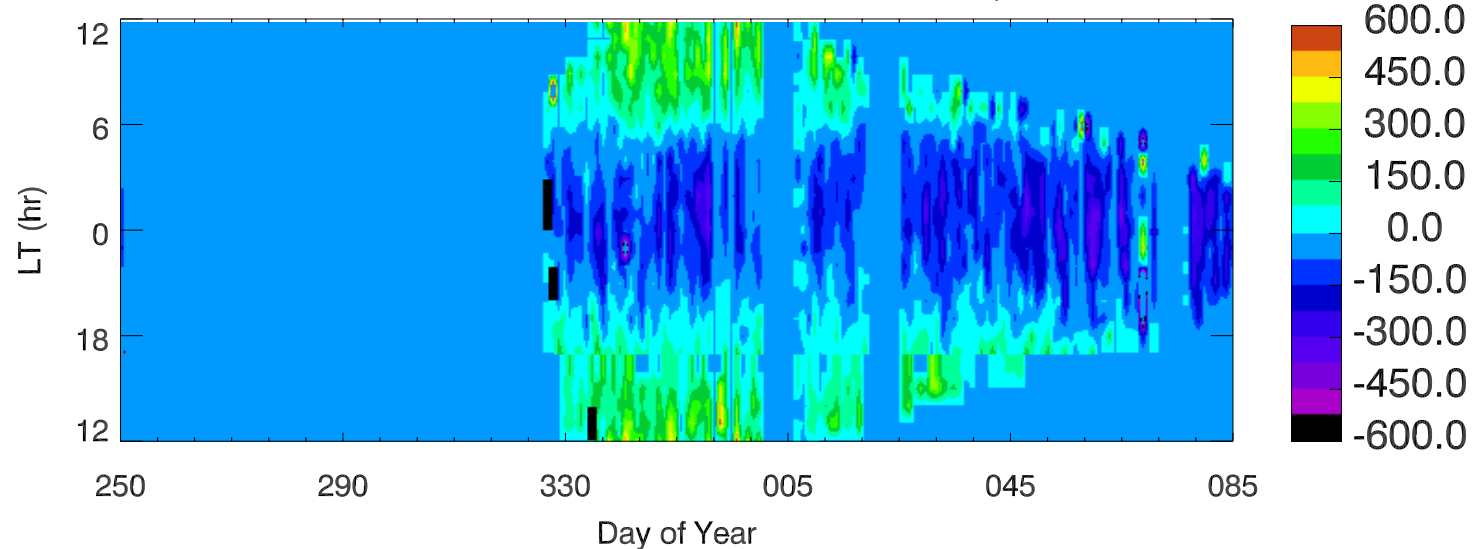
Zonal Winds Resolute O 6300 2014/15
