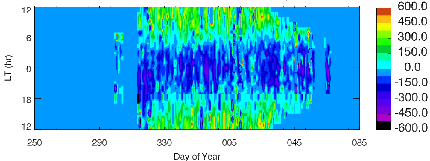
Meridional Winds Eureka O 6300 2014/15
