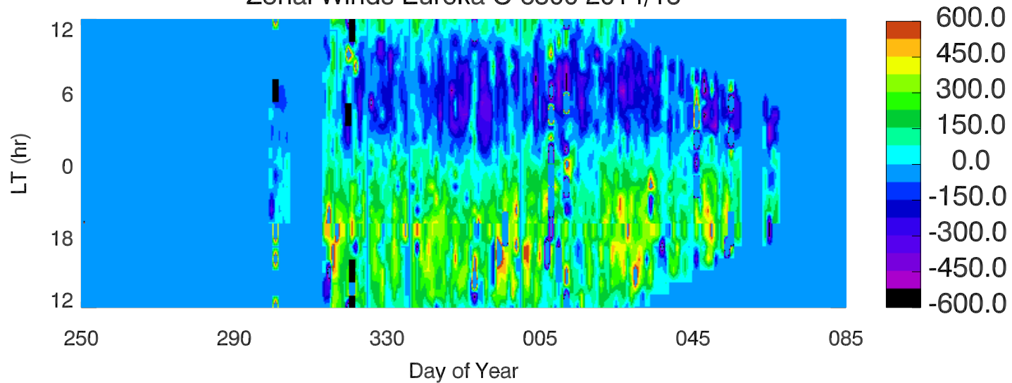
Zonal Winds Eureka O 6300 2014/15
