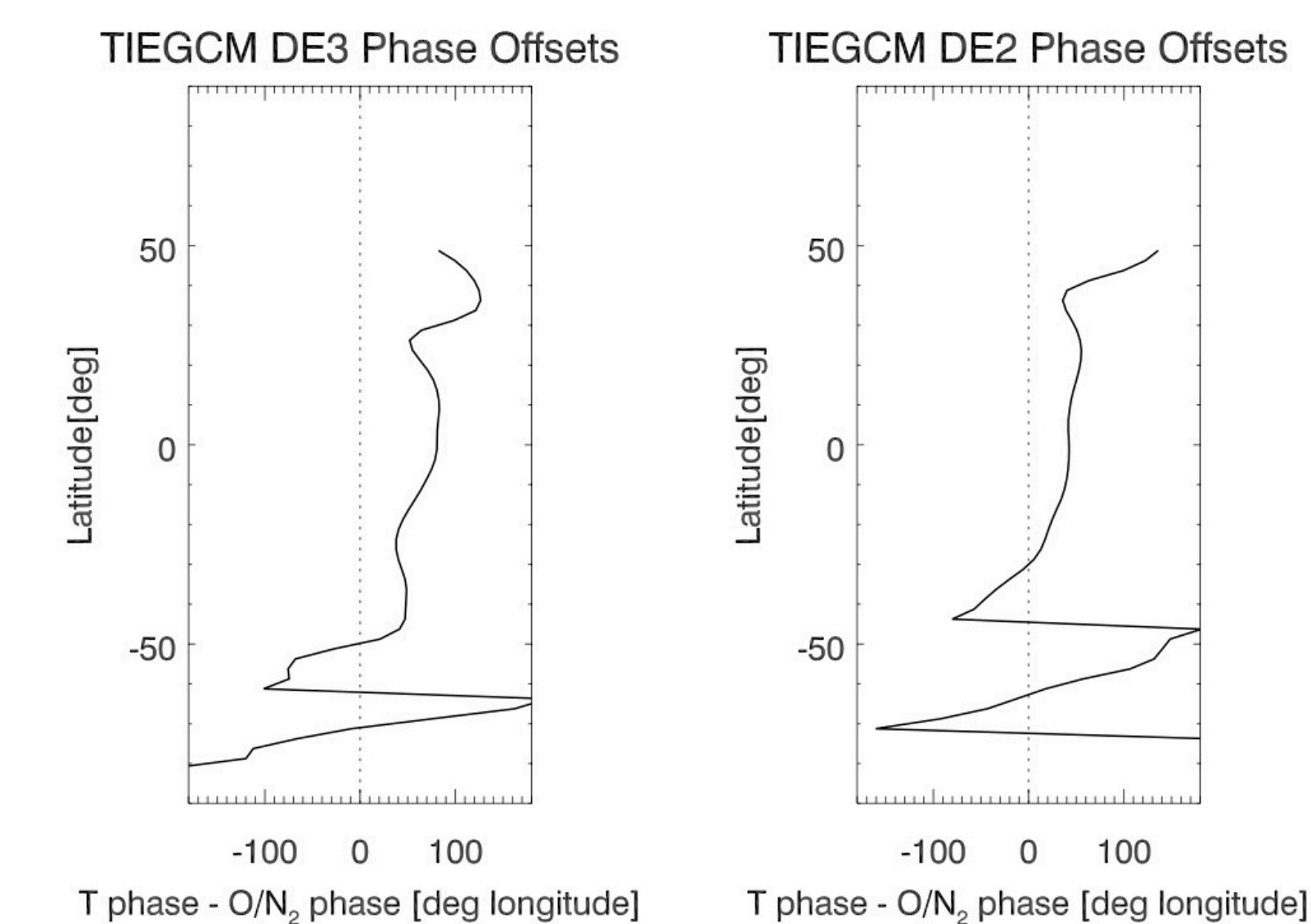
Figure 3. Expected tidal phase offsets between T and O/N 2 for DE3 and DE2 respectively in GOLD data derived from TIEGCM interfaced with the GLOW model. February solar quiet conditions. We propose to diagnose nonmigrating tides in GOLD data by using these phase offsets as functions of latitude, time-of-year, and solar conditions.
