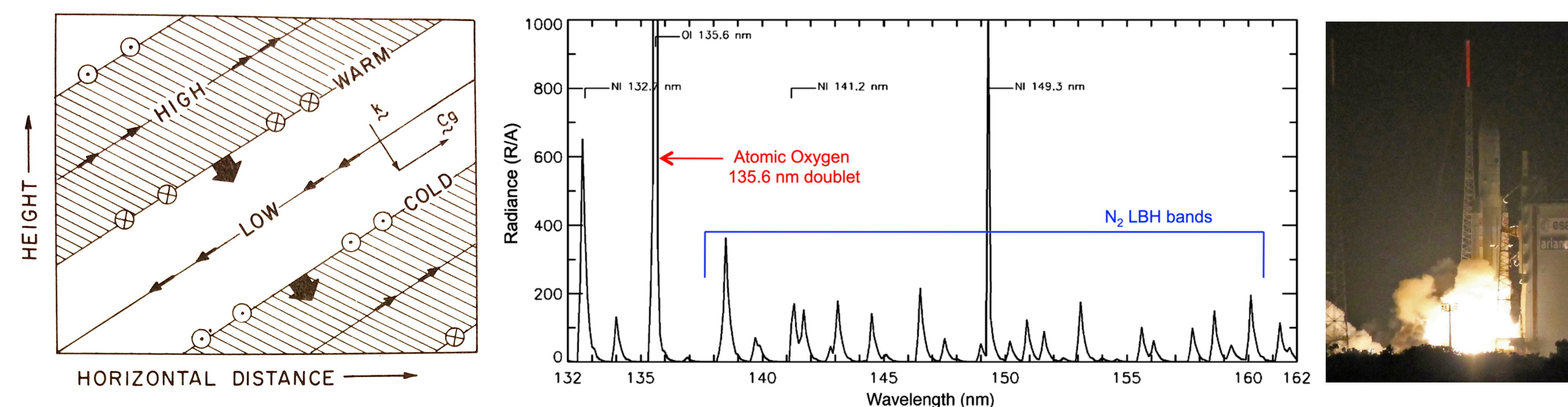
Figure 2. (left) Phase offsets between temperature, winds, and geopotential for intertio-gravity waves according to linear wave theory. Taken from Andrews (1987). (center) Daytime far-ultraviolet (FUV) model airglow spectrum at which GOLD observes. (right) Last January Ariane 5 launched with GOLD onboard SES-14 as a hosted science payload.
