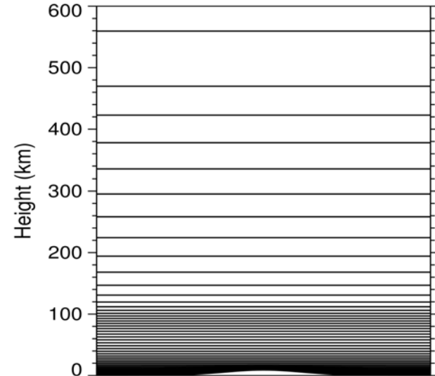
WAM hybrid vertical grid (every 3rd level)
