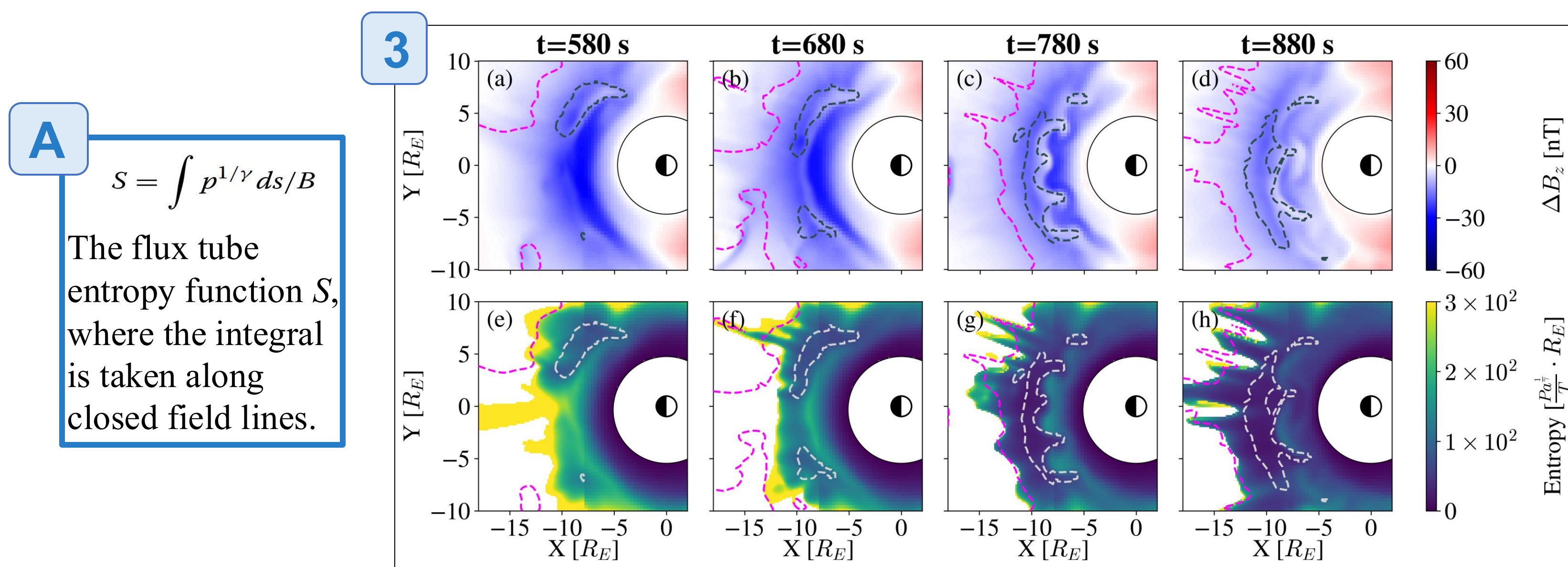
Figure 3: Panels (a-d): Residual B_z , i.e. the magnetic field minus the Earth's dipole field. Panels (e-h) flux tube entropy S . All panels are in the Z=0 plane, with \pm 400 \text{ km s}^{-1} velocities marked with grey/pink contours.
