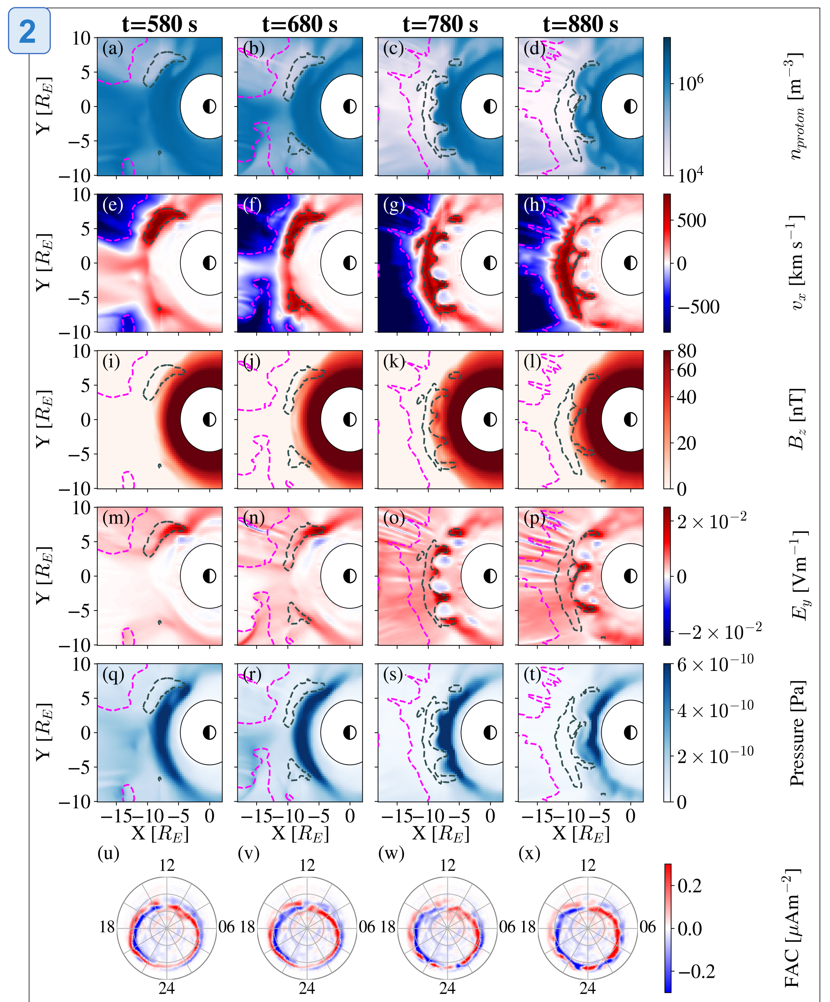
Figure 2: Panels (a-d): proton density. Panels (e-h): ion v_x . Panels (i-l) B_z , Panels (m-p) E_y . Panels (q-t) pressure. The contour lines indicate 400 km s -1 (grey) and -400 km s -1 (pink) velocities. Panels (u-x): FACs on the ionospheric grid of the simulation, in magnetic local time (MLT) coordinates.
