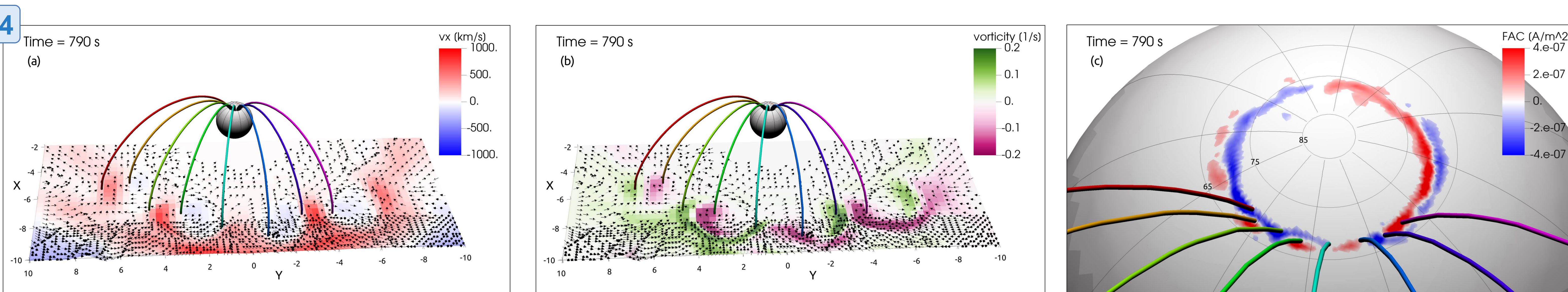
Figure 4: Panel (a): ion v_x , panel (b): the z-component of flow vorticity. Panel (c): Magnetic field lines mapped to the ionosphere, and the FAC strength on the ionospheric grid.
