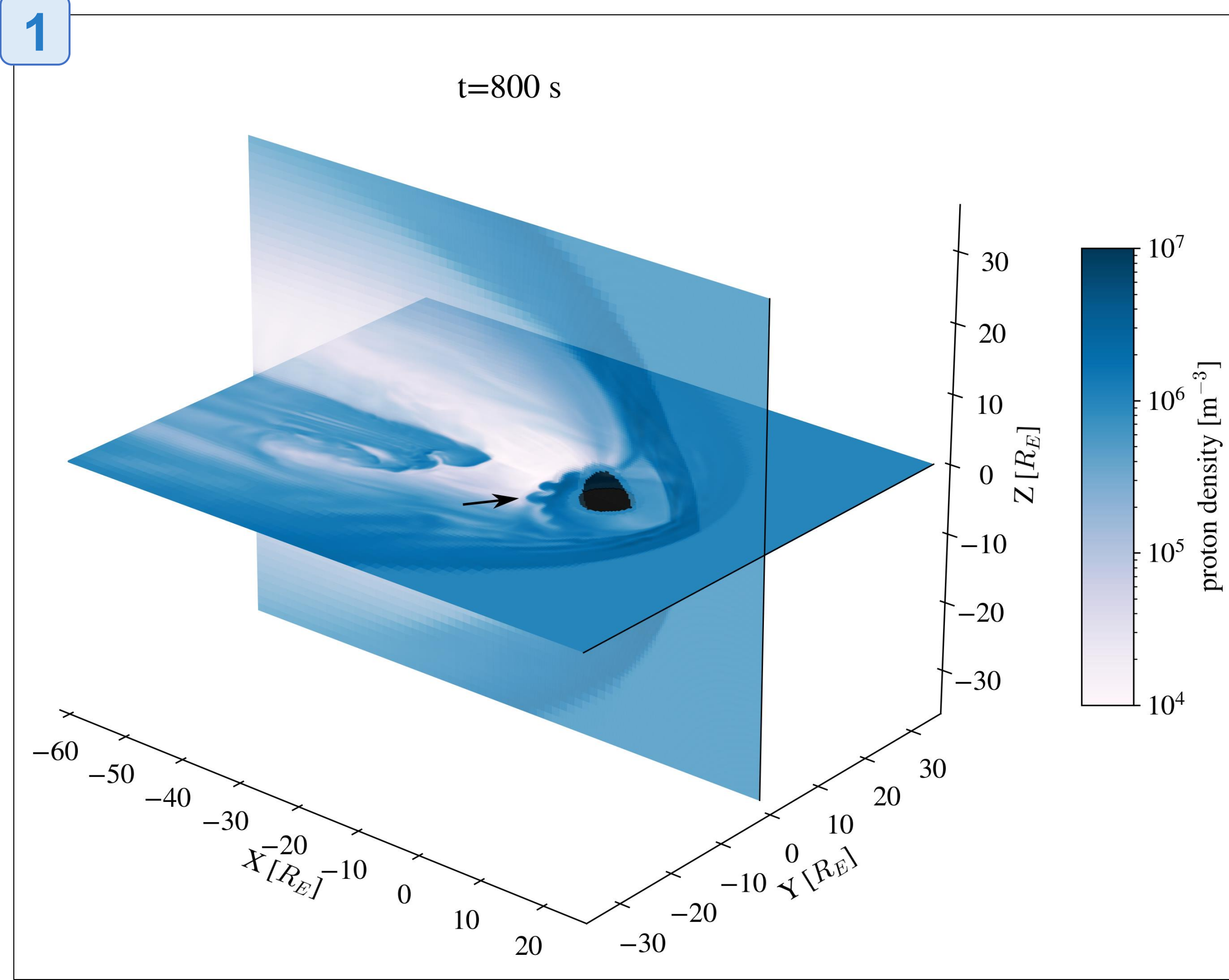
Figure 1: Proton density in the Vlasior simulation domain, the arrow points out the transition region between the dipole field and the magnetotail, where a wavy density structure forms.
